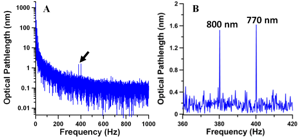
Fig. 4. (A) Power spectrum of optical pathlength ( op ) variations at a fixed 350 \mu\text{m} tissue optical depth (550 \mu\text{m} from the fiber endface). The op power spectrum was acquired by converting time domain phase data presented at the Fig. 3 to op variation [ op(t) = \varphi(t)\lambda/(4\pi) ] and using a Fast Fourier Transformation (FFT) of the first 5 s of the data. (B) Laser-induced op variations at 380 Hz (800 nm) and 400 Hz (770 nm) indicated by arrow in A.
